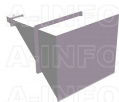
LB-650-20-C-SFSPO Standard Gain Horn Antenna 1.12-1.7GHz 20dB Gain SMA Female
