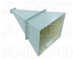
LB-650-20-A Standard Gain Horn Antenna 1.12-1.7GHz 20dB Gain Rectangular Waveguide Interface
